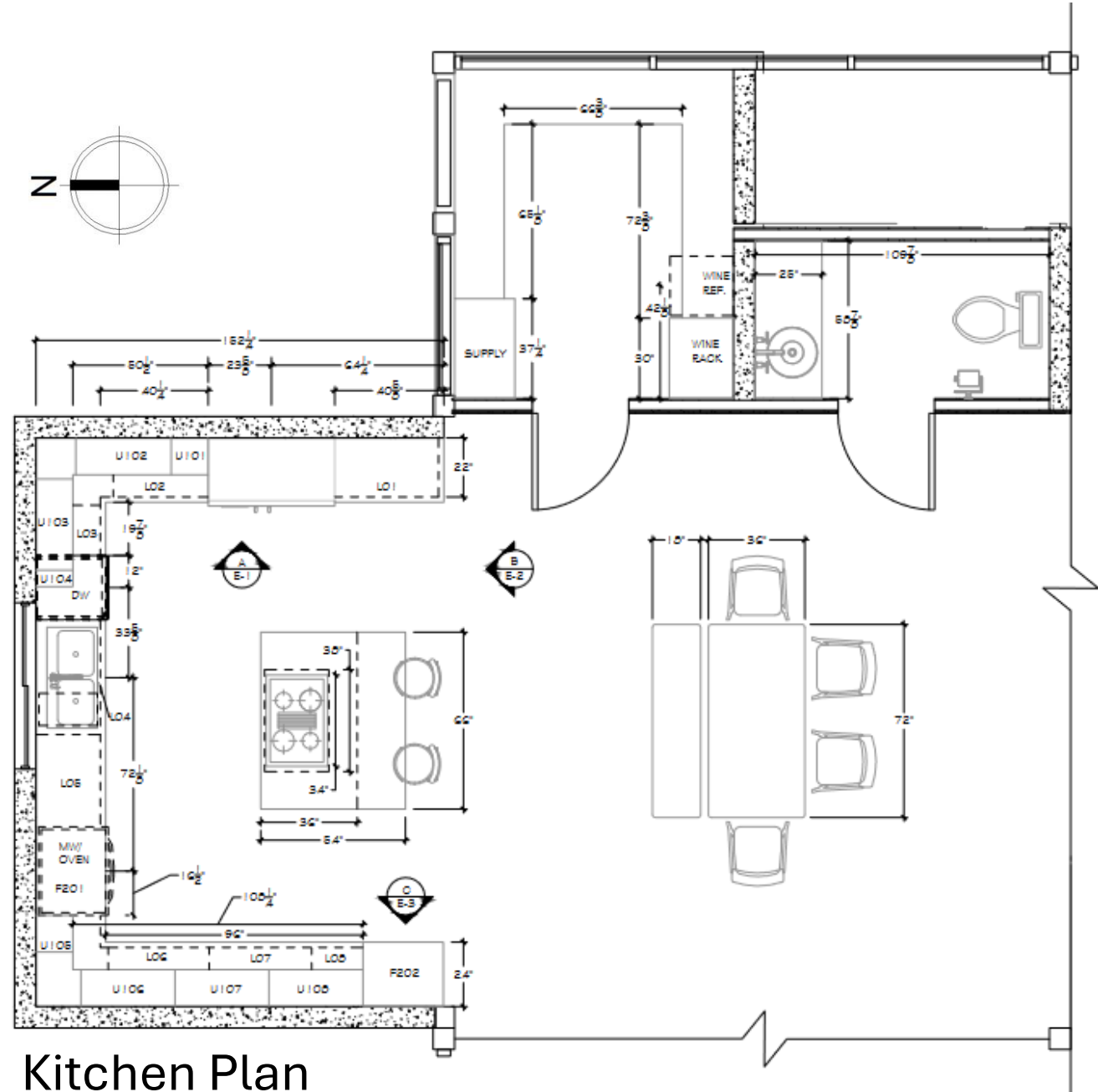
Kitchen Plan
